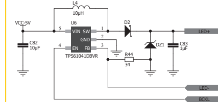
LED driver
