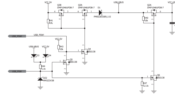
USB host
