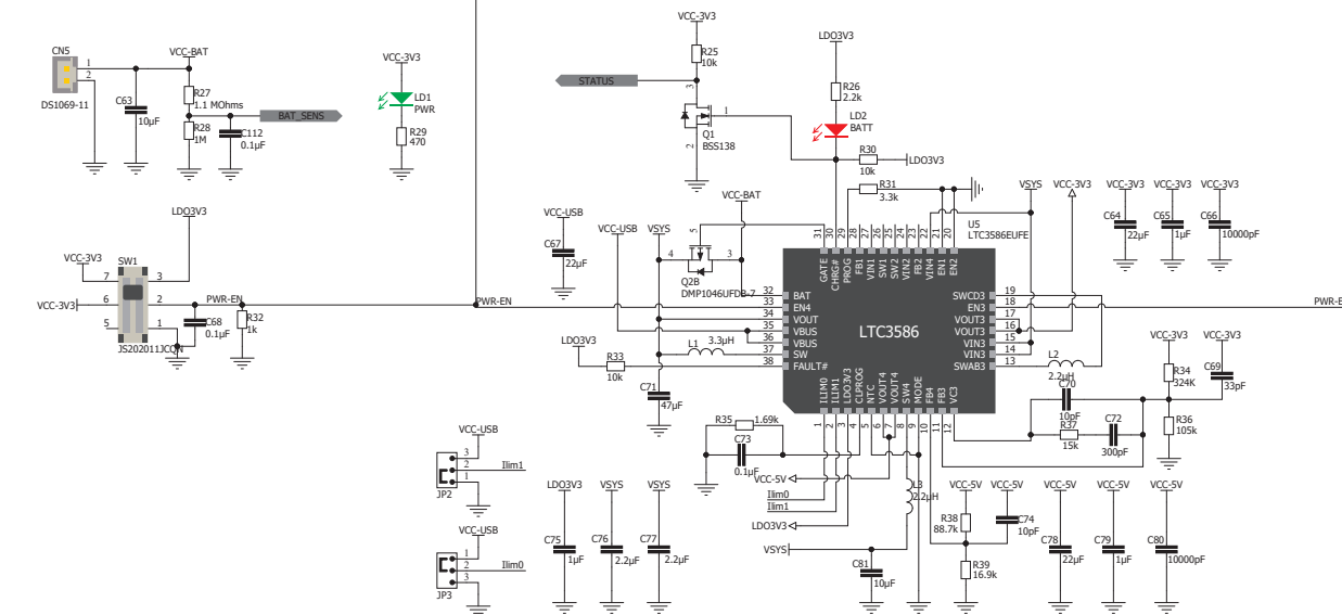
3V3 &amp; 5V Power Supply
