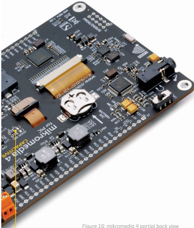
Figure 16: mikromedia 4 partial back view
