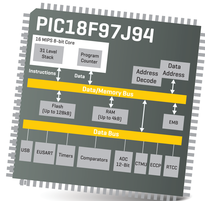
Figure 1: PIC18F97J94 MCU block schematic
