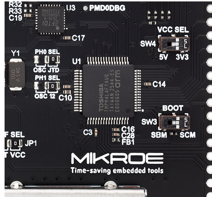
Figure 2: TPM4L4FYAUG MCU
