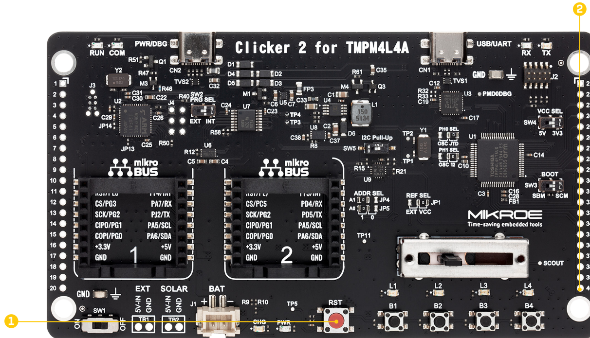
Figure 4: Clicker 2 for TPM4L4A front view
