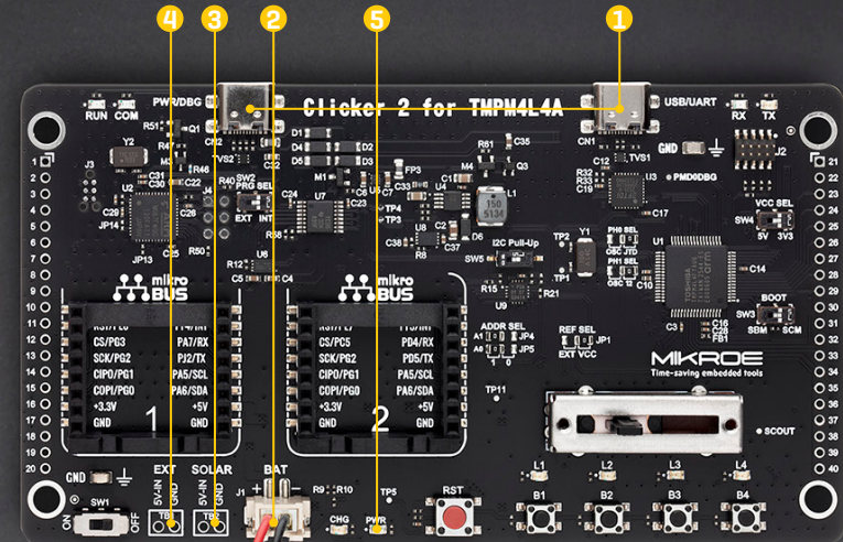
Figure 6: Power supply view
