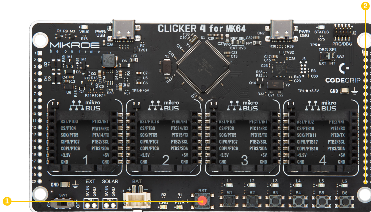
Figure 4: Clicker 4 for MK64 front view
