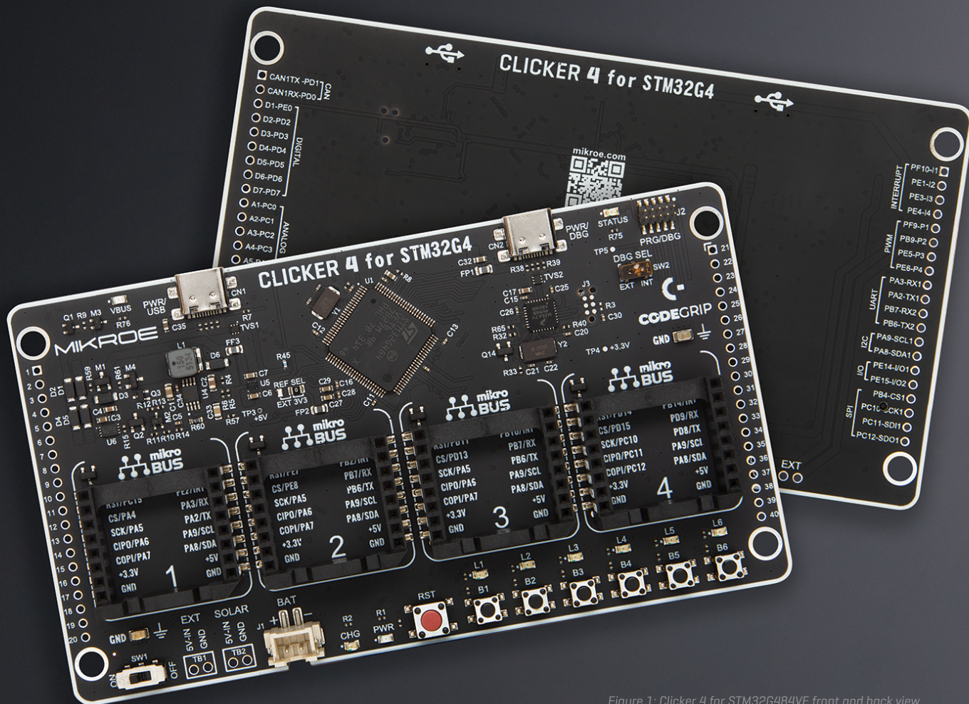
Figure 1: Clicker 4 for STM32G484VE front and back view
