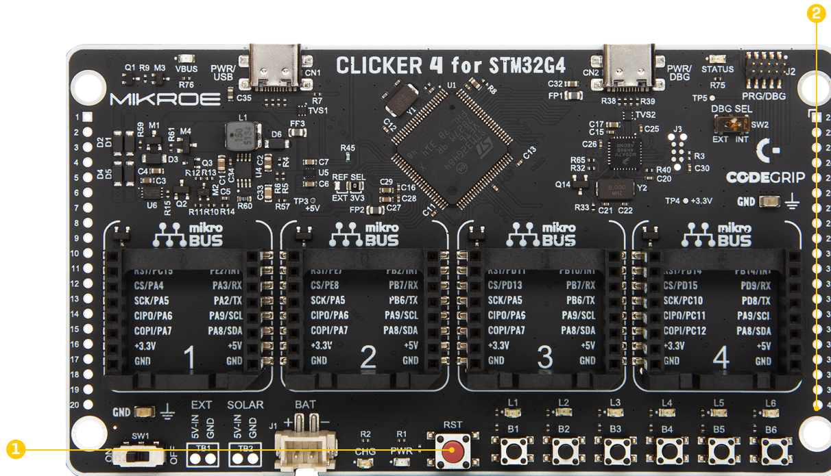
Figure 4: Clicker 4 for STM32G4 front view
