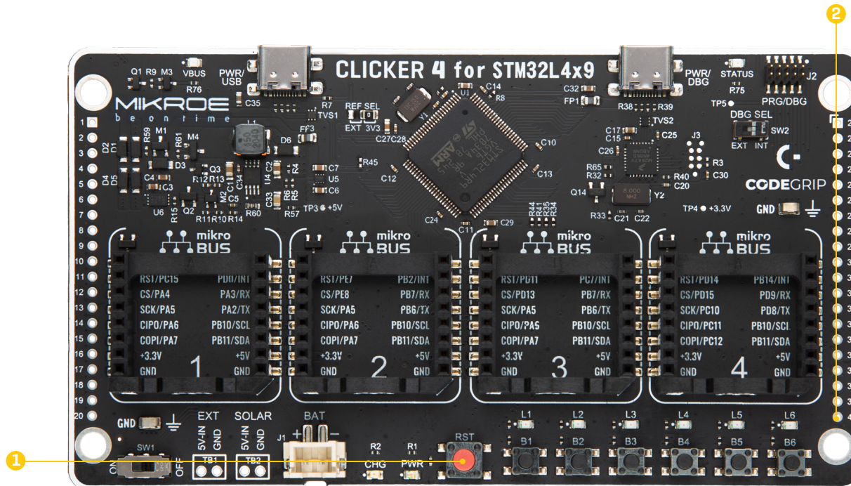
Figure 4: Clicker 4 for STM32L4x9 front view
